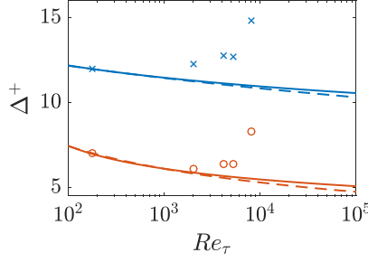
FIG. 5. The grid resolution required to resolve 99% of the wall-shear stress events. Blue lines: \Delta x^+ . Red lines: \Delta z^+ . Solid lines: Assuming \sigma^+ \sim \log(\text{Re}_\tau) . Dashed lines: Assuming \sigma^+ \sim \log(\text{Re}_\tau) . Cross symbols: \Delta x^+ in some of the channel flow DNSs. Round symbols: \Delta z^+ in some of the channel flow DNSs. The references are as follows: For \text{Re}_\tau = 180 , Ref. [3]; for \text{Re}_\tau = 2000 , Refs. [41,48]; for \text{Re}_\tau = 4200 , Ref. [42]; for \text{Re}_\tau = 5200 , Ref. [41]; and for \text{Re}_\tau = 8000 , Ref. [49].
