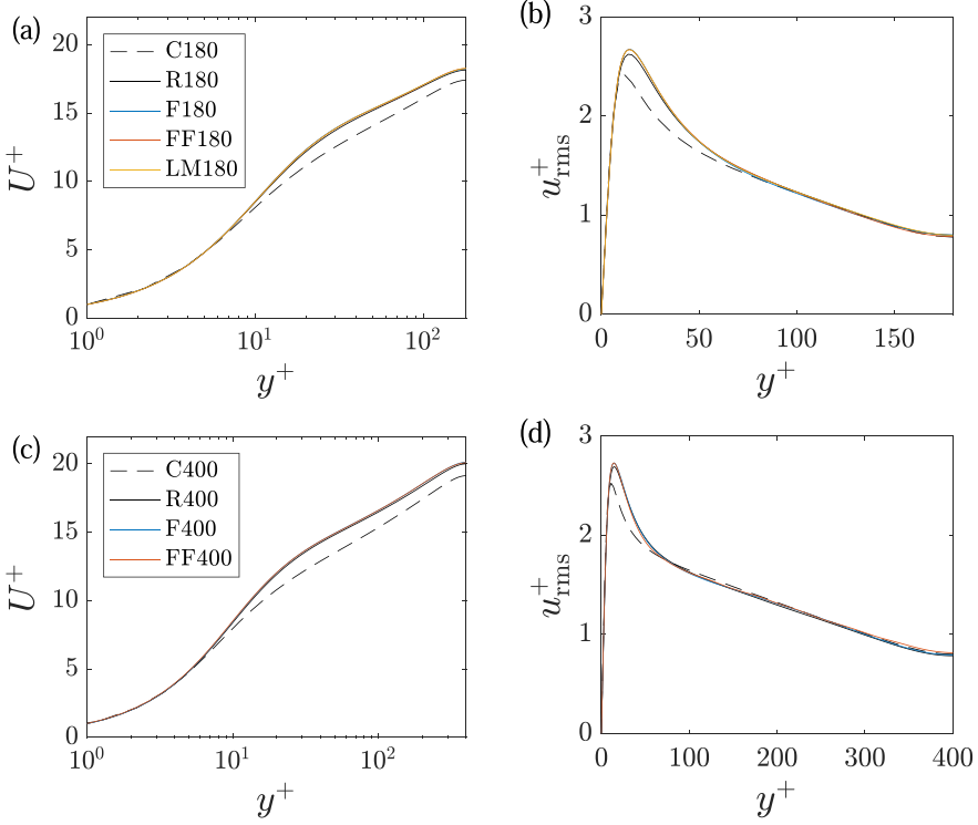
FIG. 1. (a), (c) Mean velocity. (b), (d) Streamwise velocity's rms. (a), (b) Results at \text{Re}_\tau = 180 (c), (d) Results at \text{Re}_\tau = 400 .
